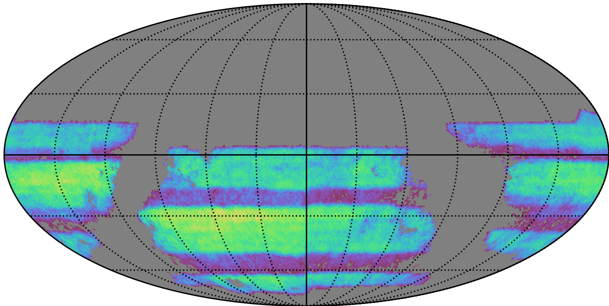
octo_v3.4_10yrs i band non-DD year 6: ExgalM5WithCuts
