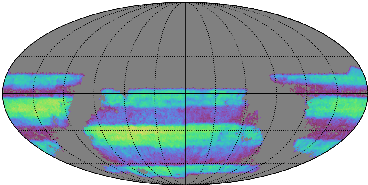
octo_v3.4_10yrs i band non-DD year 5: ExgalM5WithCuts
