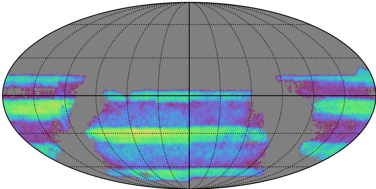
octo_v3.4_10yrs i band non-DD year 4: ExgalM5WithCuts
