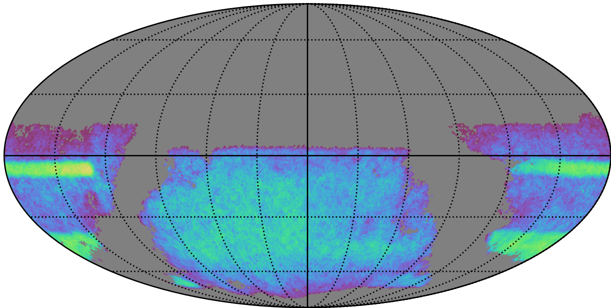
octo_v3.4_10yrs i band non-DD year 2: ExgalM5WithCuts
