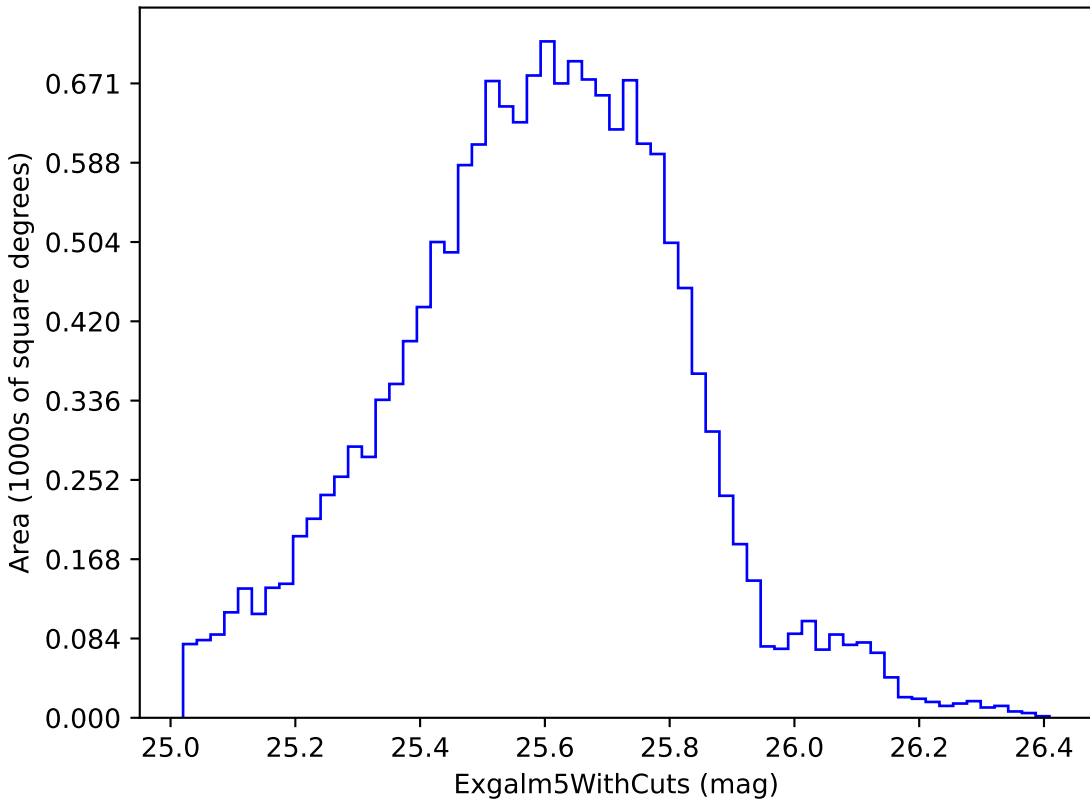
octo_v3.4_10yrs i band non-DD year 2: ExgalM5WithCuts
