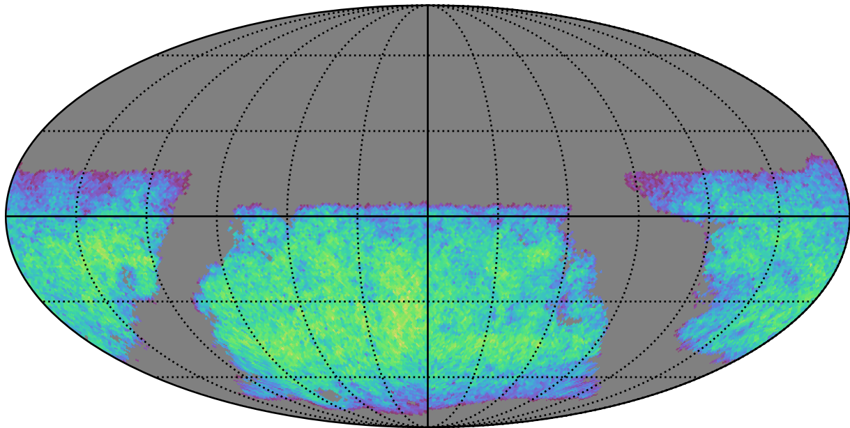
octo_v3.4_10yrs i band non-DD year 1: Exgalm5WithCuts
