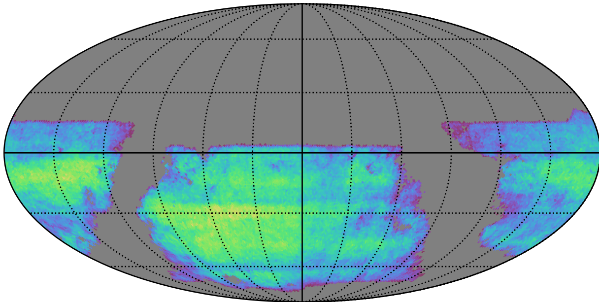
octo_v3.4_10yrs i band non-DD year 10: ExgalM5WithCuts
