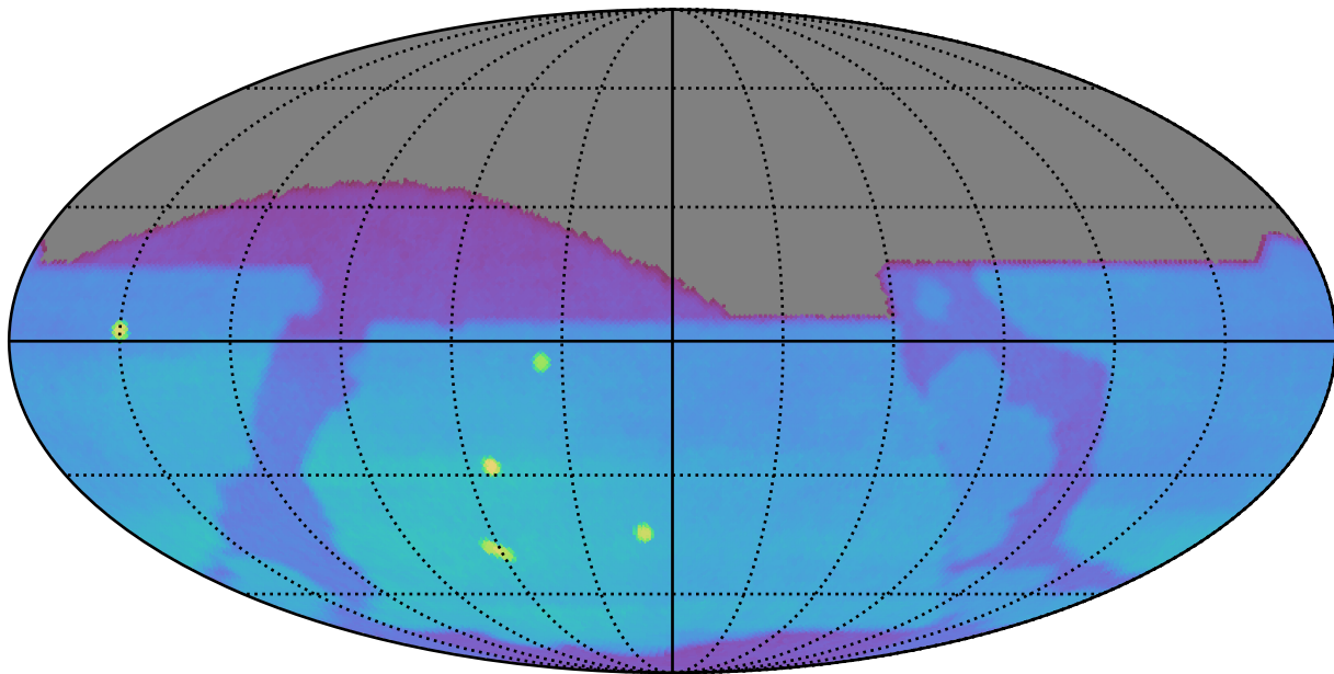
octo_v3.4_10yrs : Brown Dwarf, L4
