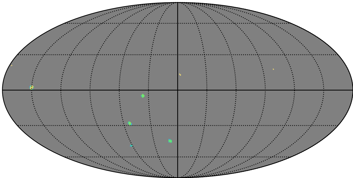
octo_v3.4_10yrs z band: AGN_TimeLag_5_days
