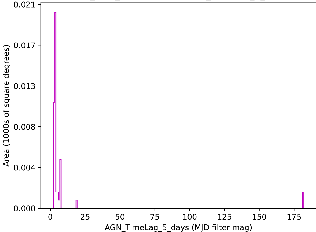
octo_v3.4_10yrs z band: AGN_TimeLag_5_days
