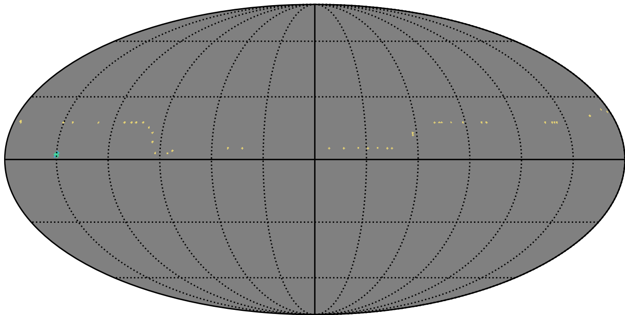
octo_v3.4_10yrs y band: AGN_TimeLag_5_days
