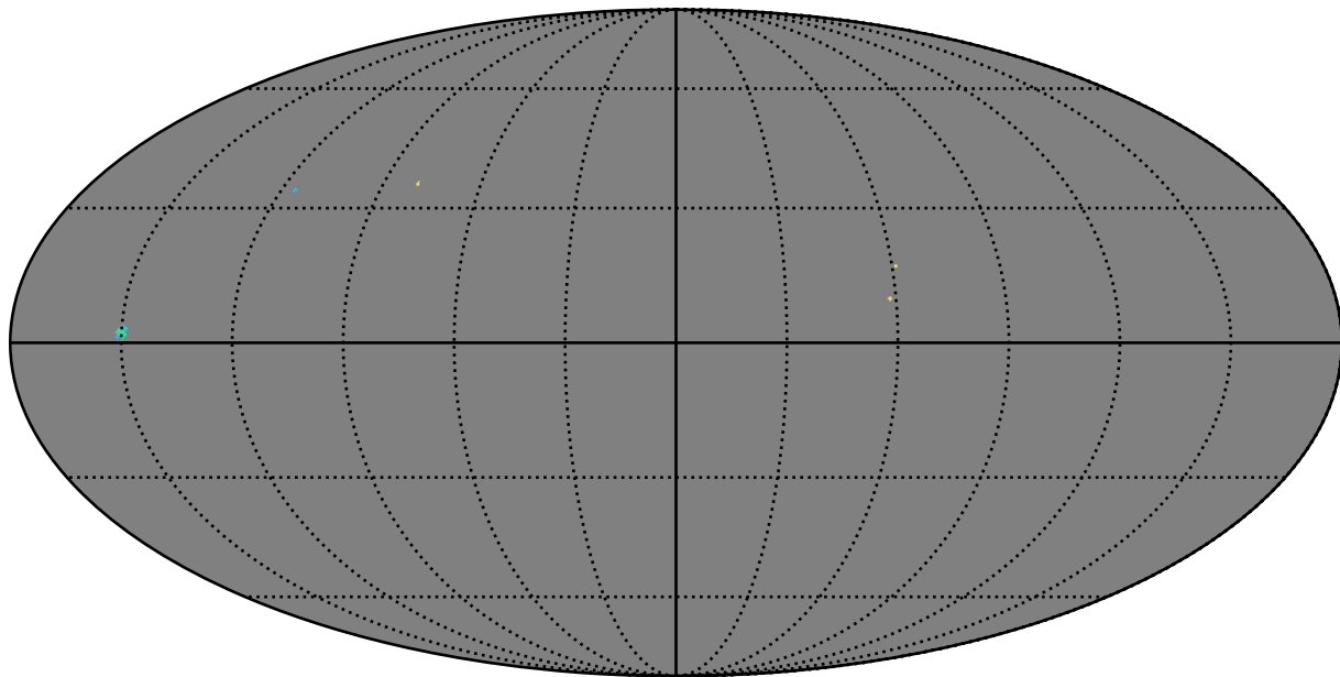
octo_v3.4_10yrs g band: AGN_TimeLag_5_days
