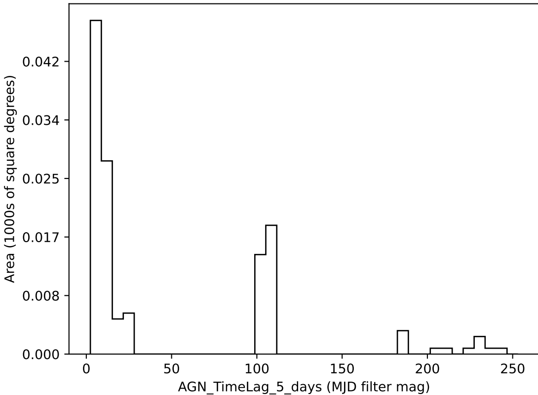
octo_v3.4_10yrs all bands: AGN_TimeLag_5_days
