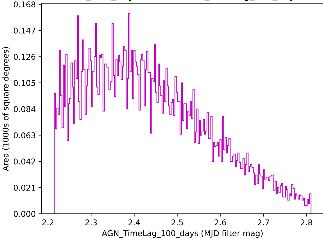
octo_v3.4_10yrs z band: AGN_TimeLag_100_days
