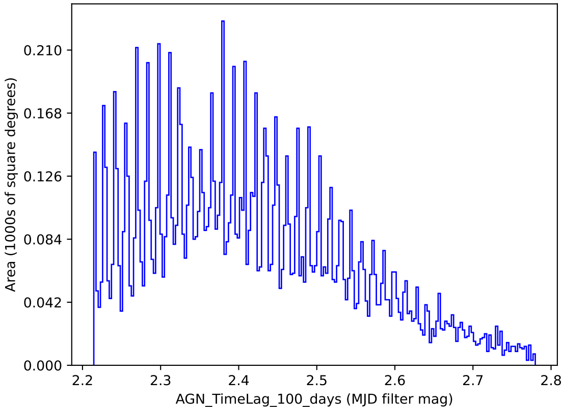
octo_v3.4_10yrs y band: AGN_TimeLag_100_days
