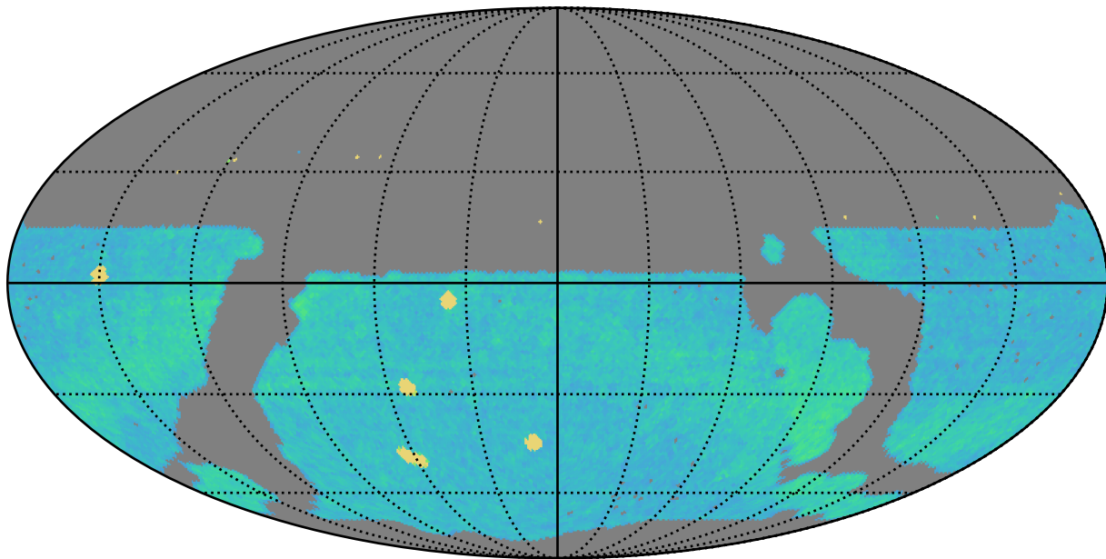
octo_v3.4_10yrs r band: AGN_TimeLag_100_days
