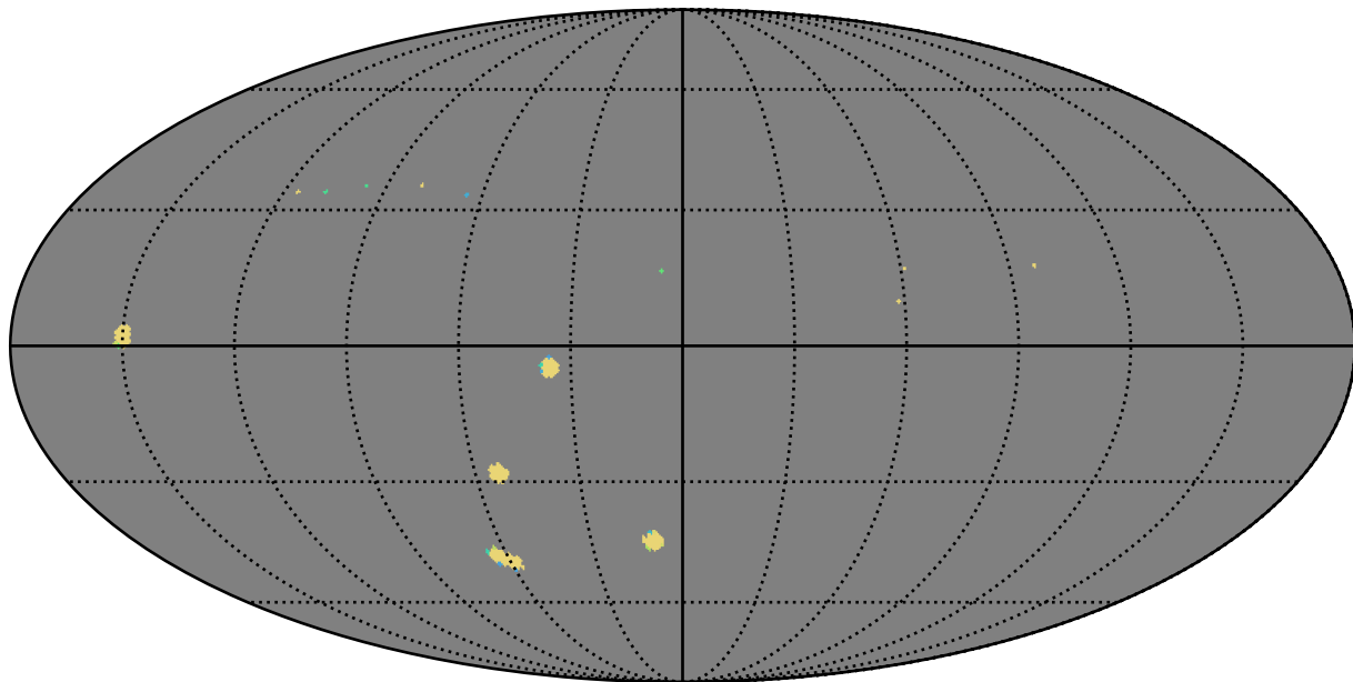
octo_v3.4_10yrs g band: AGN_TimeLag_100_days
