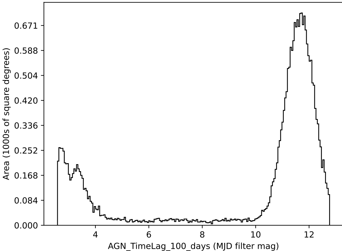
octo_v3.4_10yrs all bands: AGN_TimeLag_100_days
