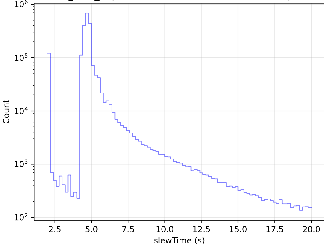
octo_v3.4_10yrs All visits: Zoom Slew Time Histogram
