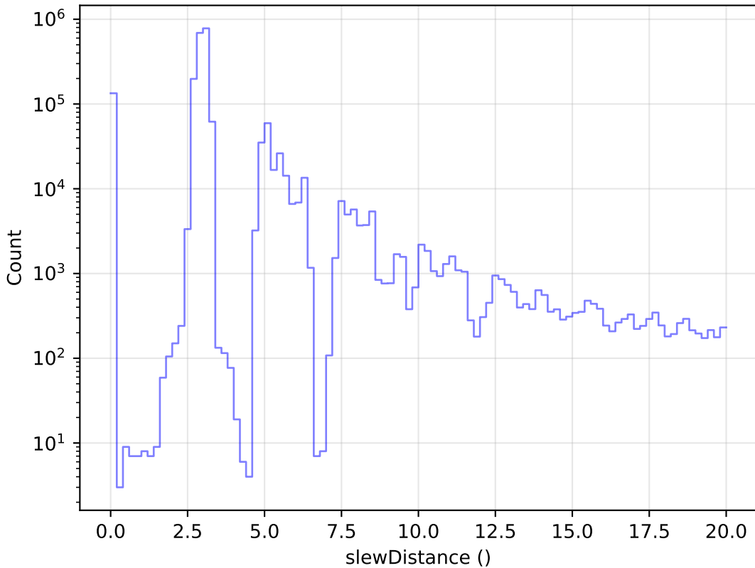
octo_v3.4_10yrs All visits: Zoom Slew Distance Histogram
