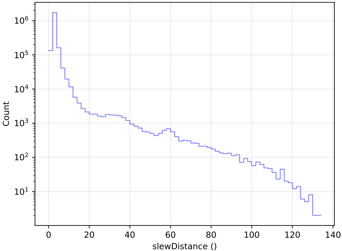
octo_v3.4_10yrs All visits: Slew Distance Histogram
