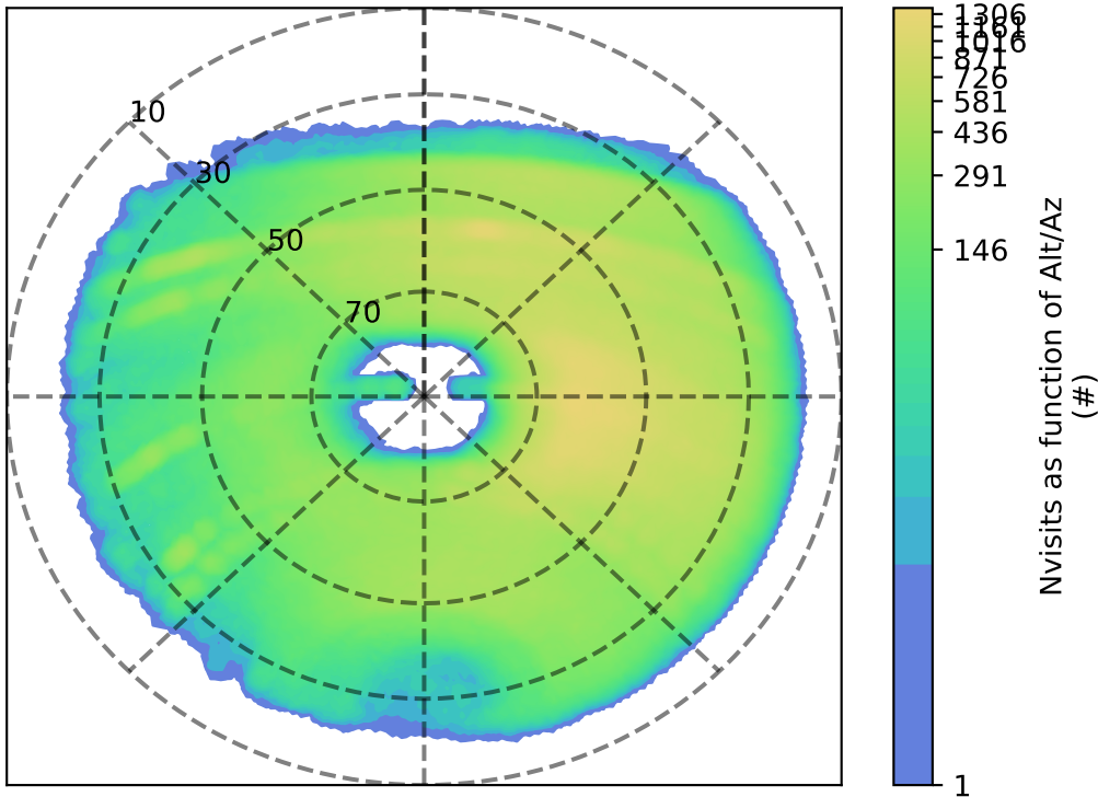
octo_v3.4_10yrs y: Nvisits as function of Alt/Az
