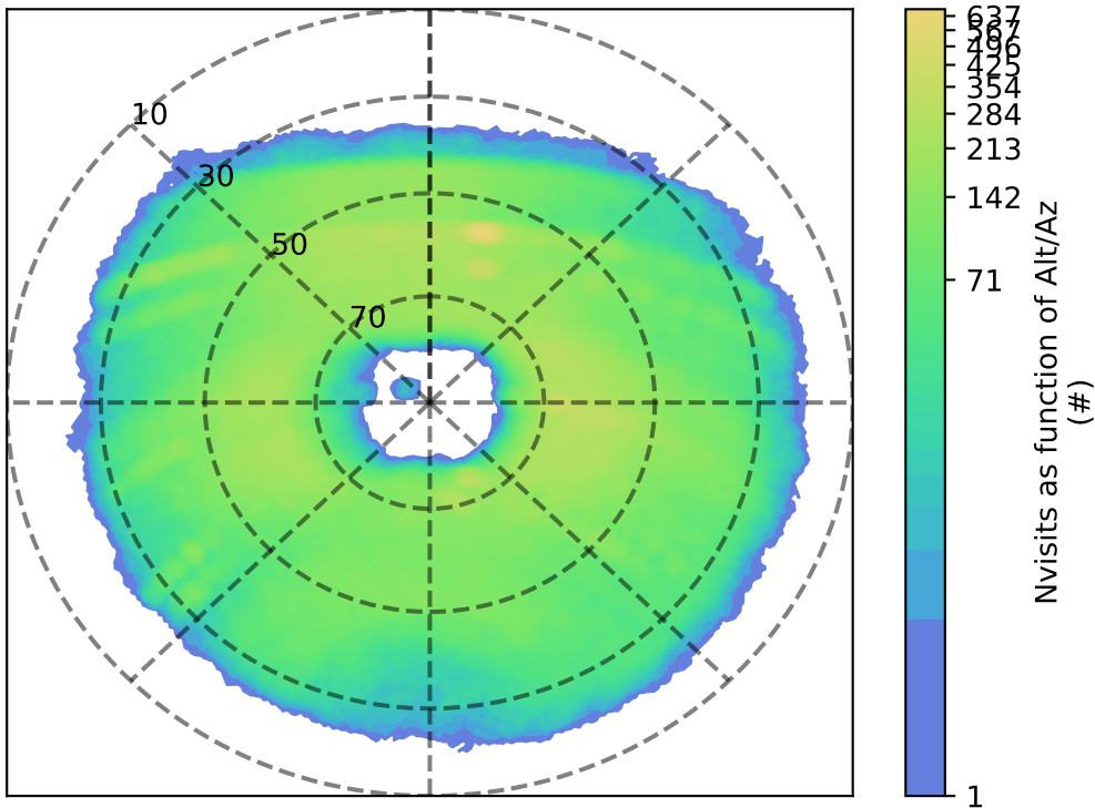
octo_v3.4_10yrs u: Nvisits as function of Alt/Az
