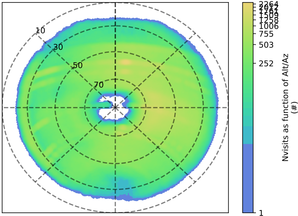
octo_v3.4_10yrs r: Nvisits as function of Alt/Az
