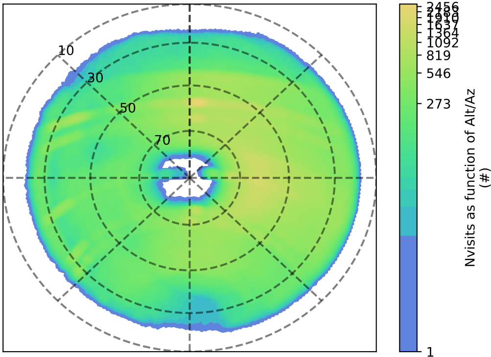
octo_v3.4_10yrs i: Nvisits as function of Alt/Az
