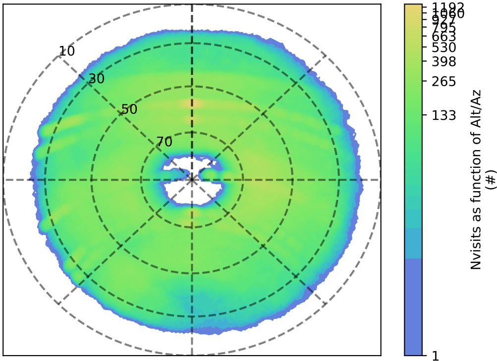
octo_v3.4_10yrs g: Nvisits as function of Alt/Az
