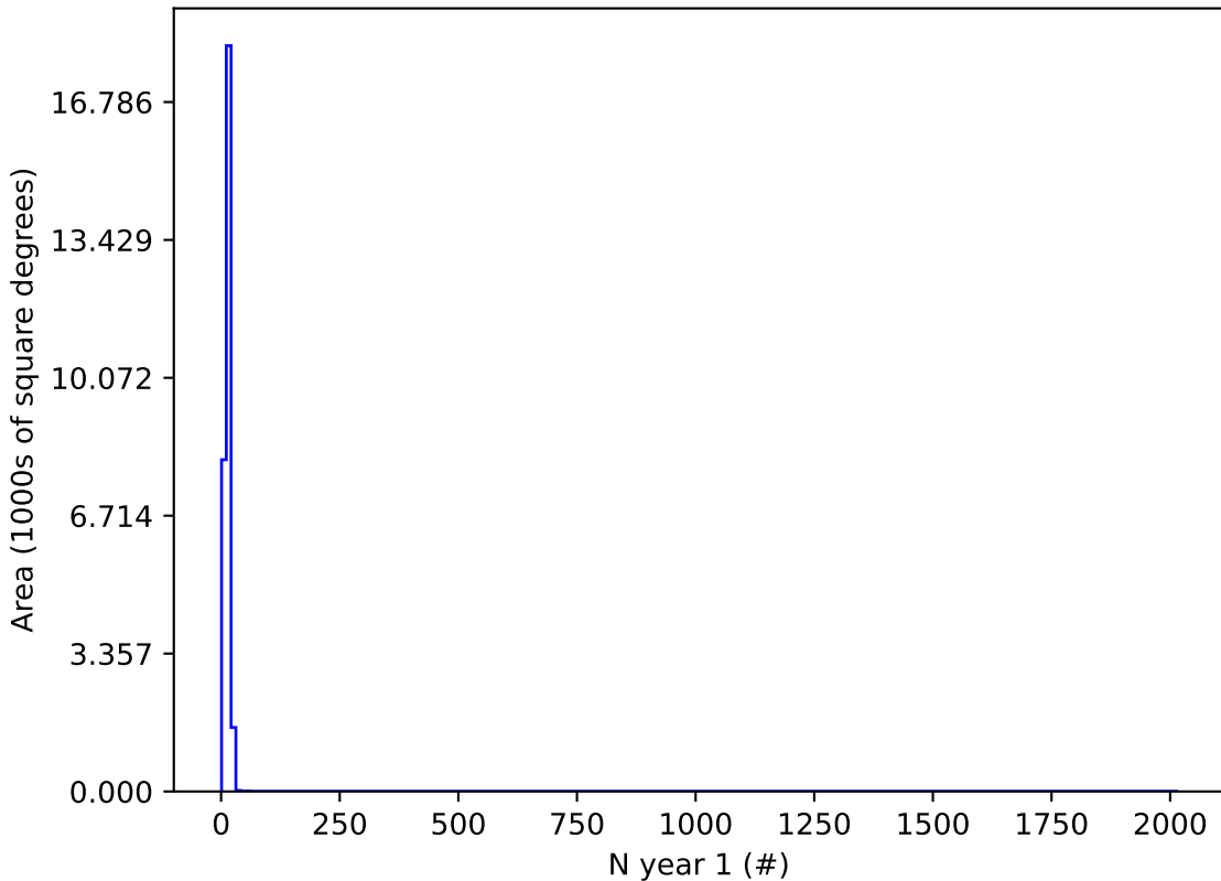
octo_v3.4_10yrs z and night < 365: N year 1
