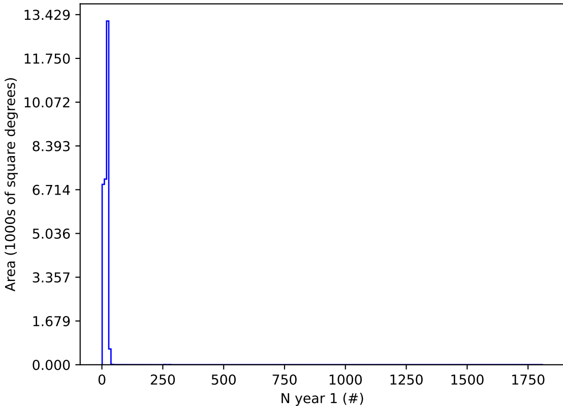
octo_v3.4_10yrs i and night < 365: N year 1
