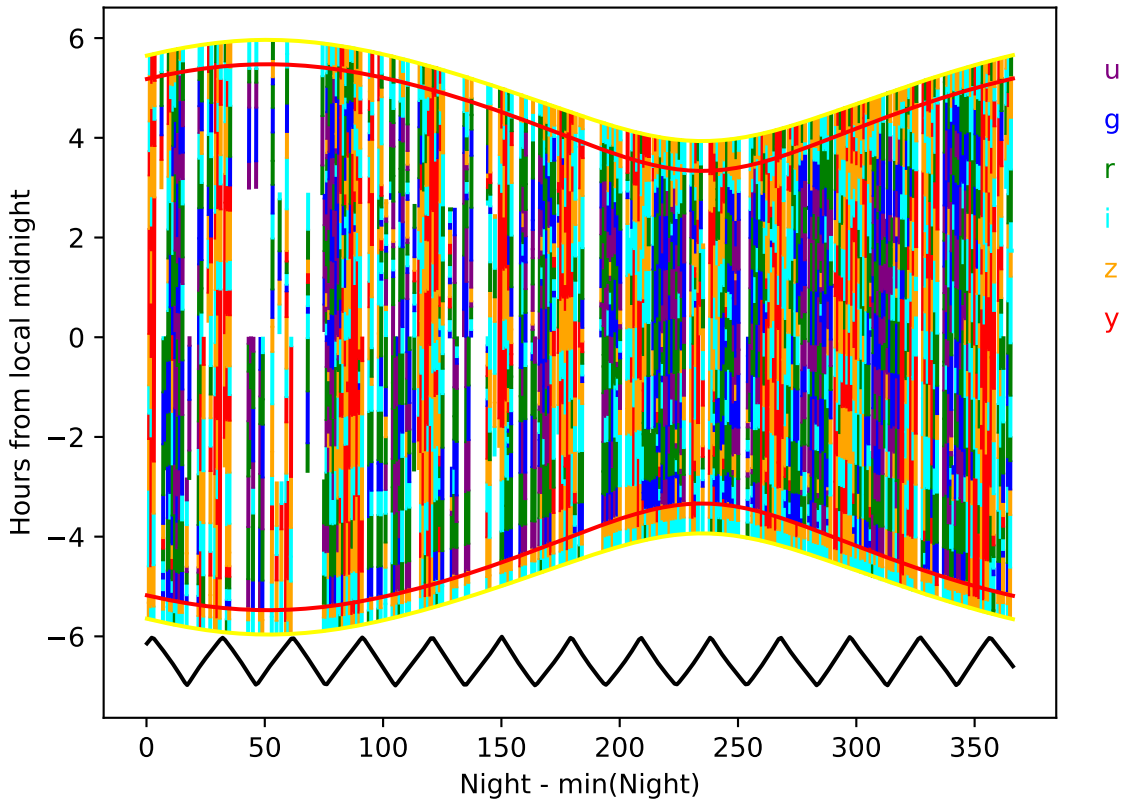
octo_v3.4_10yrs year 9-10: Hourglass
