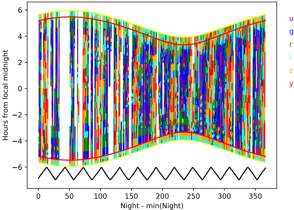
octo_v3.4_10yrs year 8-9: Hourglass
