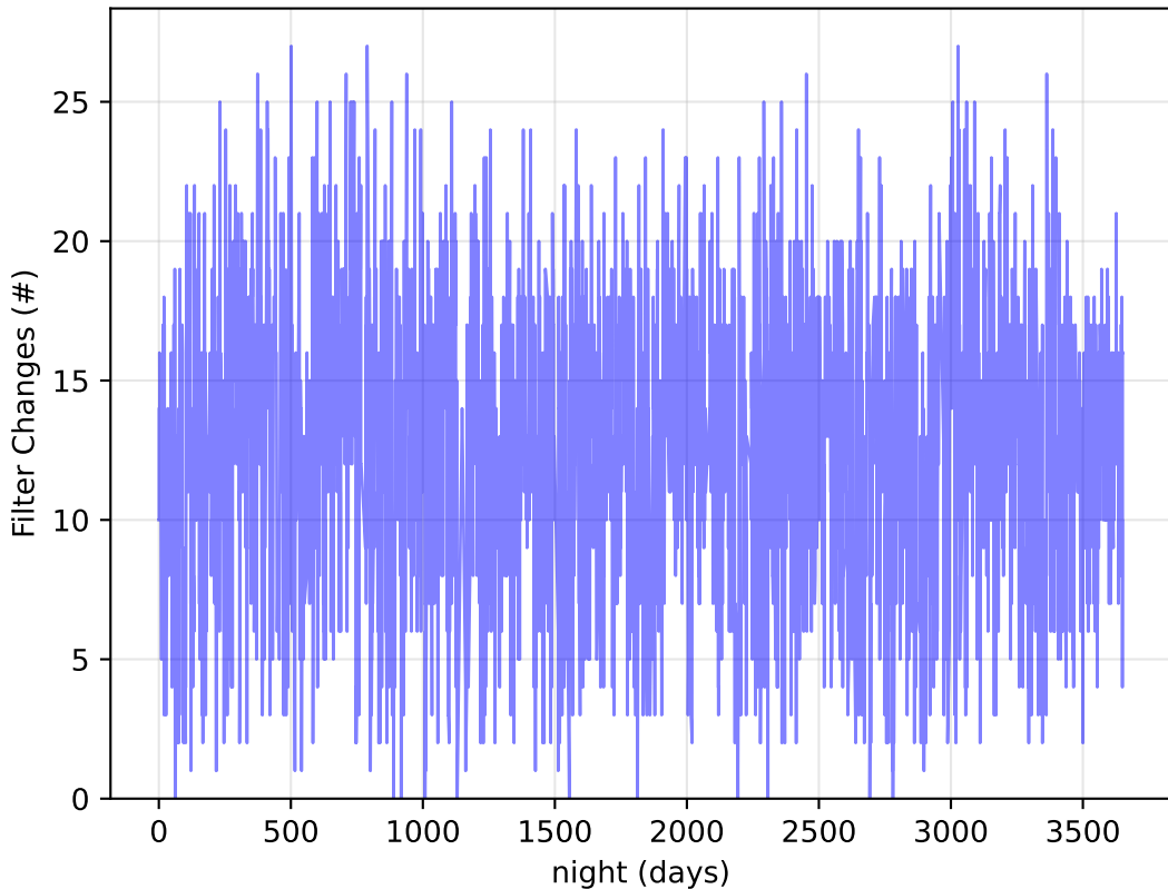
octo_v3.4_10yrs : Filter Changes
