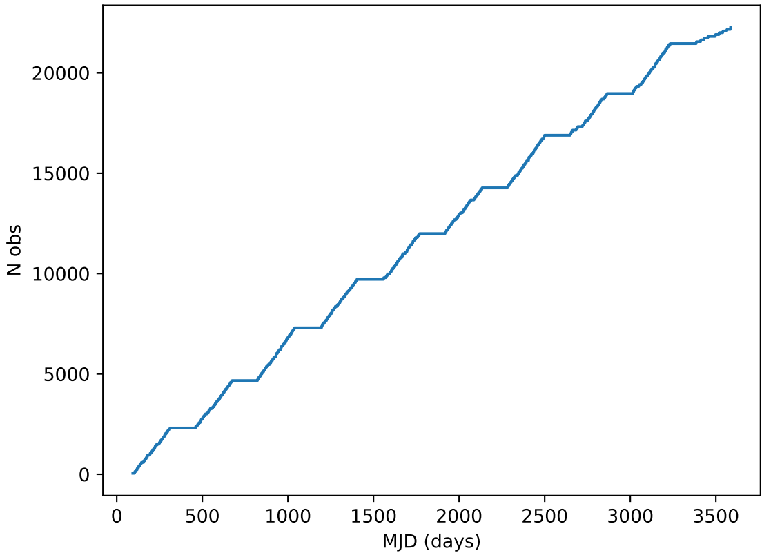
octo_v3.4_10yrs note like DD:ECDFS%: Cumulative
