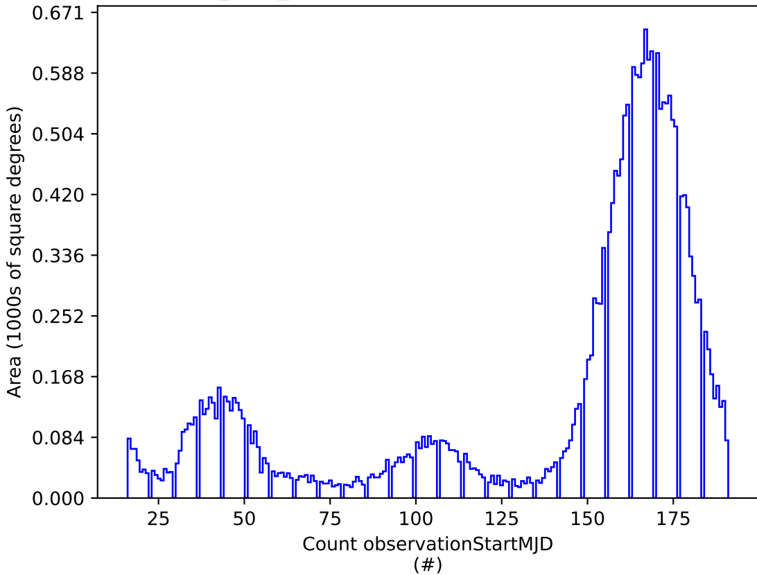
octo_v3.4_10yrs y: Count observationStartMJD
