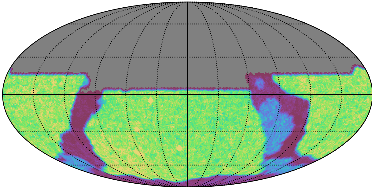
octo_v3.4_10yrs u: Count observationStartMJD
