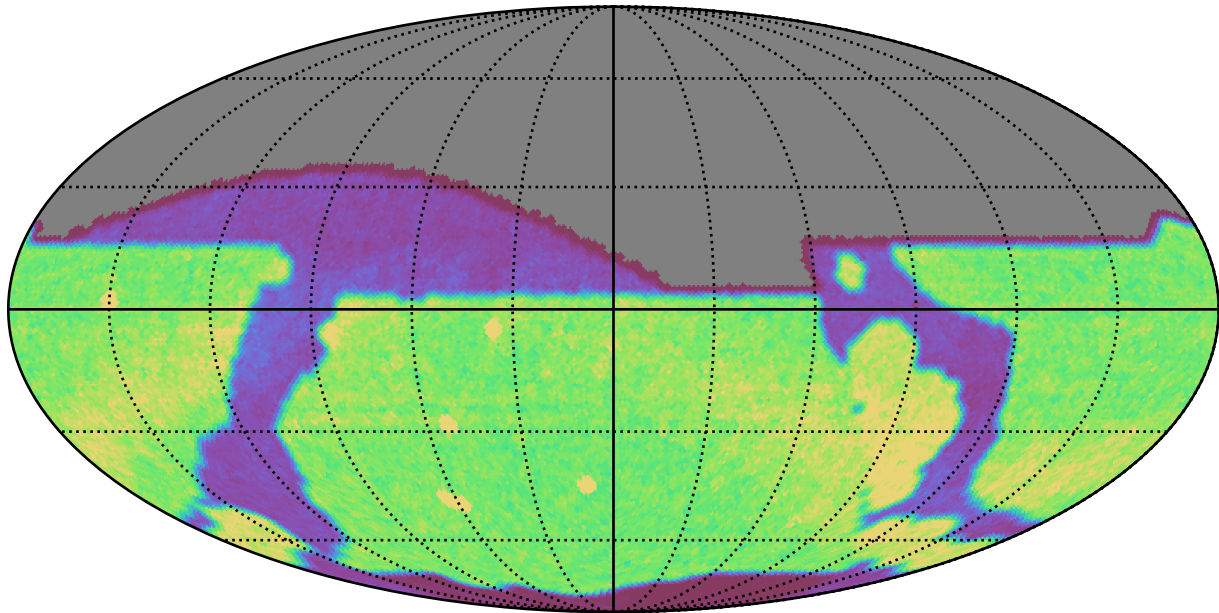
octo_v3.4_10yrs r: Count observationStartMJD
