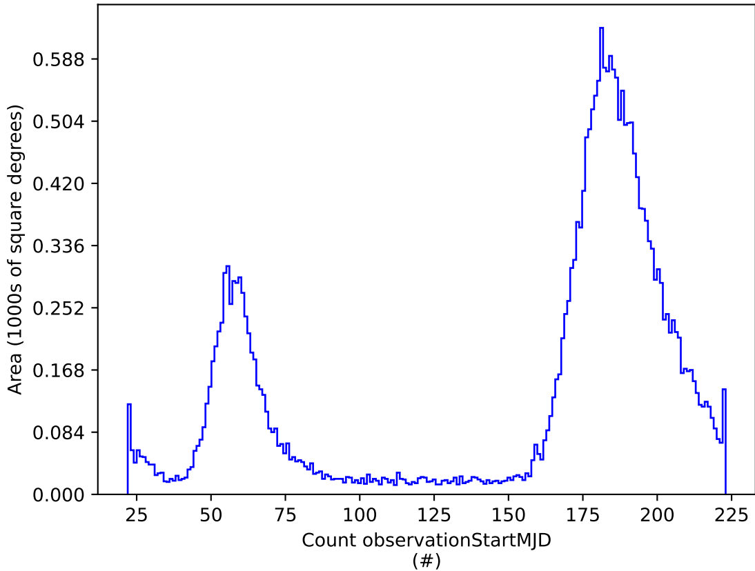
octo_v3.4_10yrs r: Count observationStartMJD
