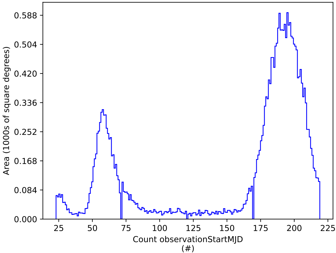
octo_v3.4_10yrs i: Count observationStartMJD
