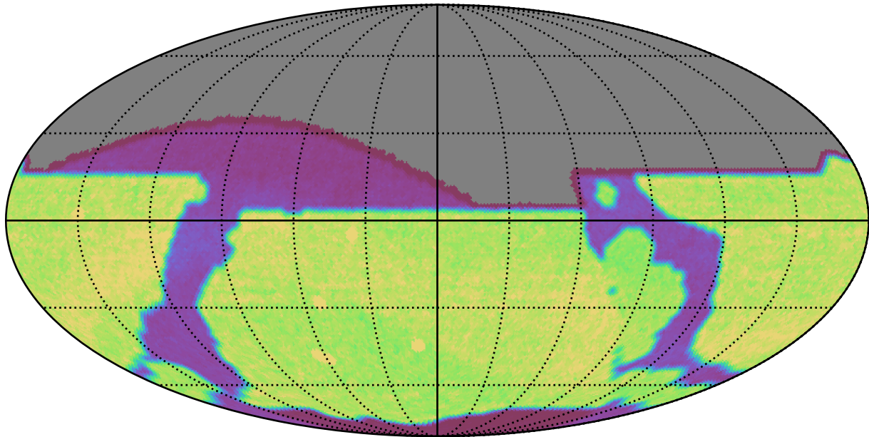
octo_v3.4_10yrs : Count observationStartMJD
