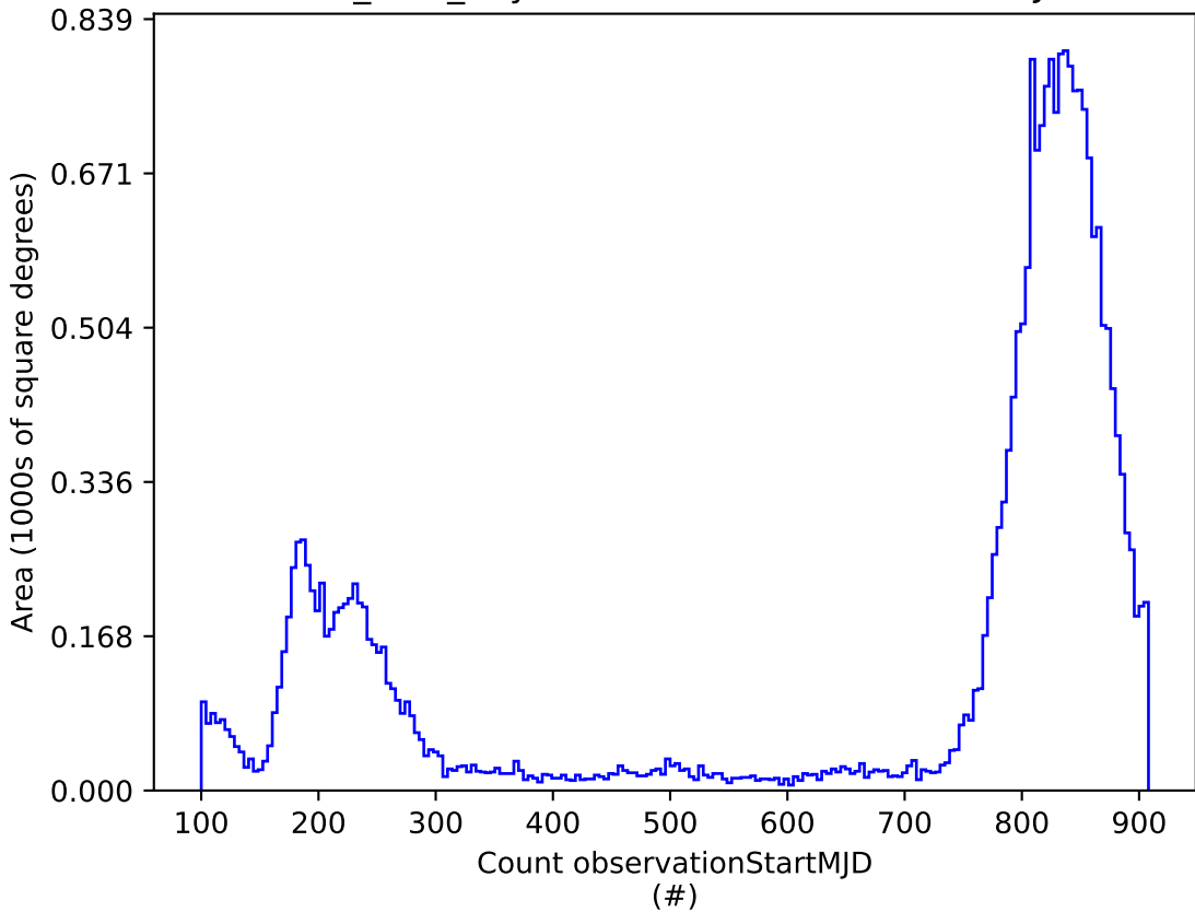
octo_v3.4_10yrs : Count observationStartMJD
