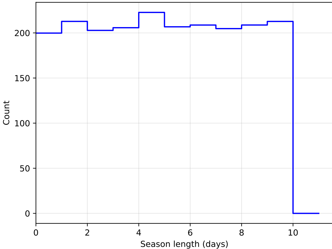
octo_v3.4_10yrs DD:XMM_LSS all bands: SeasonLength
