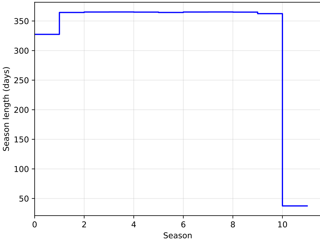
octo_v3.4_10yrs DD:WFD all bands: SeasonLength
