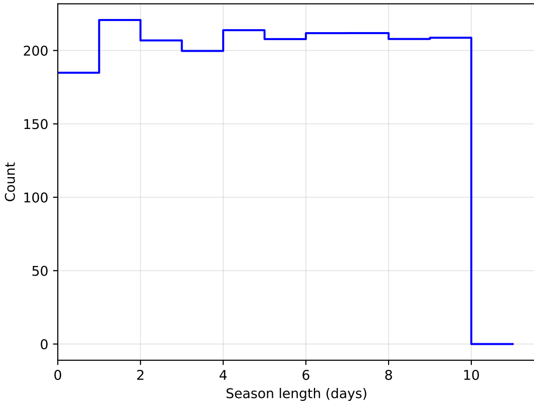
octo_v3.4_10yrs DD:ELAISS1 all bands: SeasonLength
