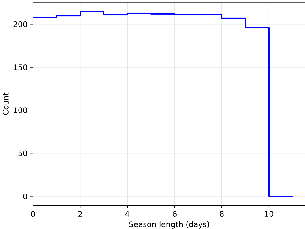
octo_v3.4_10yrs DD:EDFS all bands: SeasonLength
