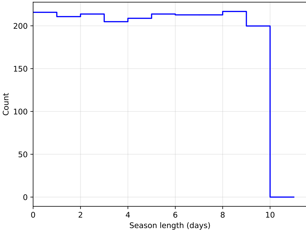
octo_v3.4_10yrs DD:ECDFS all bands: SeasonLength
