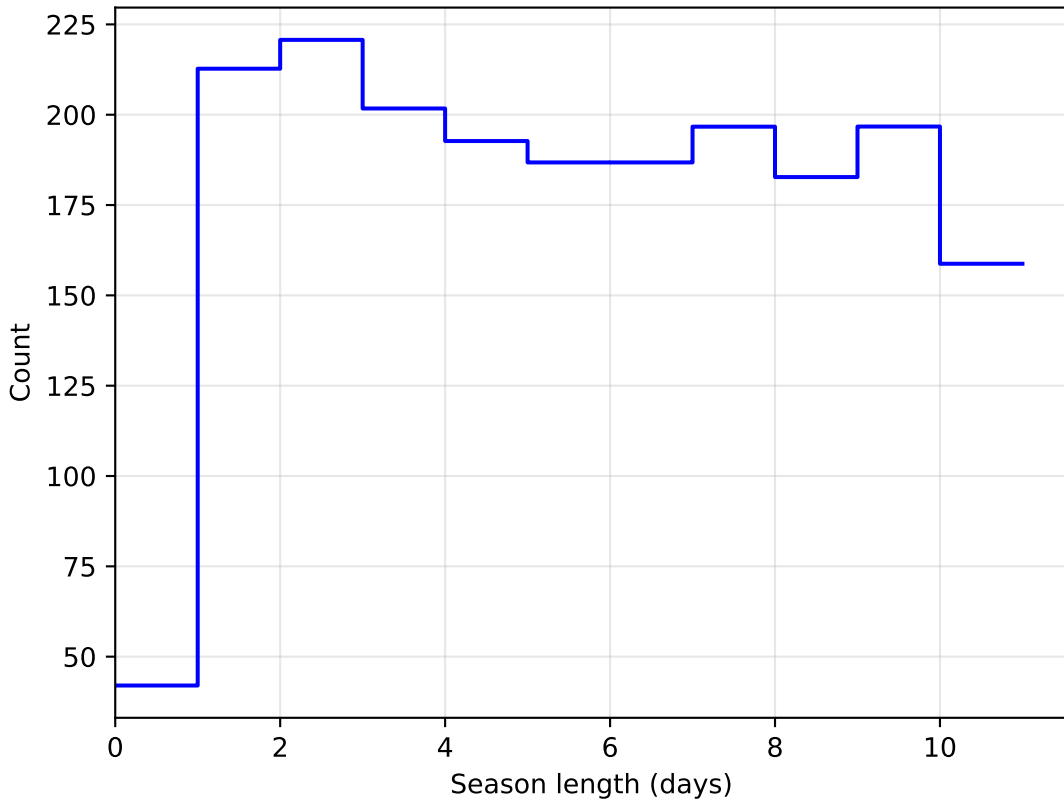
octo_v3.4_10yrs DD: COSMOS all bands: SeasonLength
