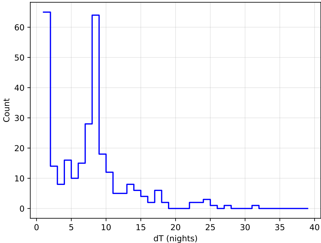
octo_v3.4_10yrs all bands: DD:XMM_LSS Delta Nights Histogram
