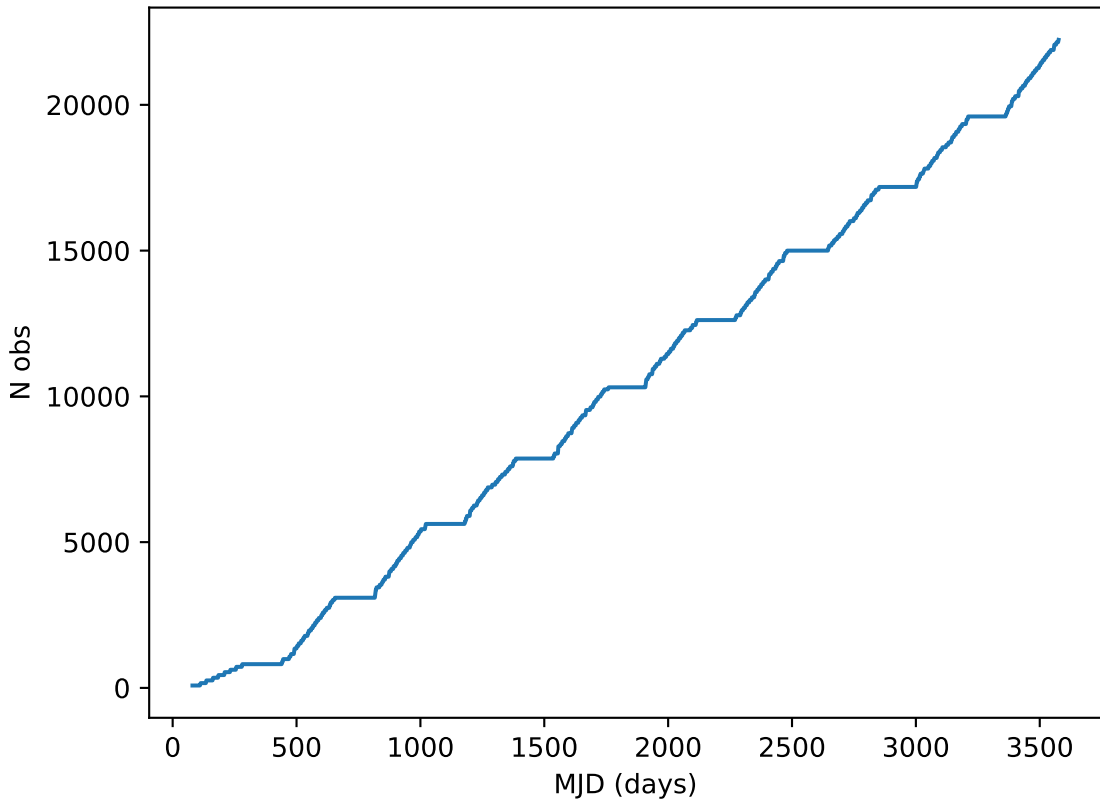
octo_v3.4_10yrs all bands: DD:XMM_LSS Cumulative NVisits
