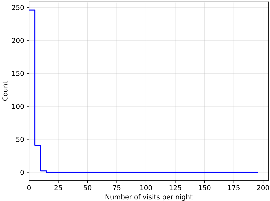
octo_v3.4_10yrs all bands: DD:WFD NVisitsPerNight
