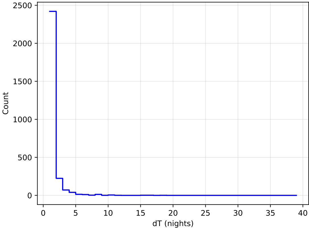
octo_v3.4_10yrs all bands: DD:WFD Delta Nights Histogram
