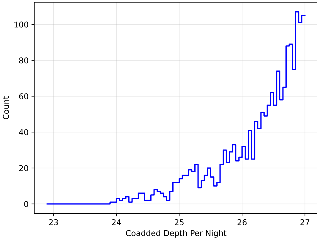
octo_v3.4_10yrs r band: DD:WFD CoaddM5PerNight
